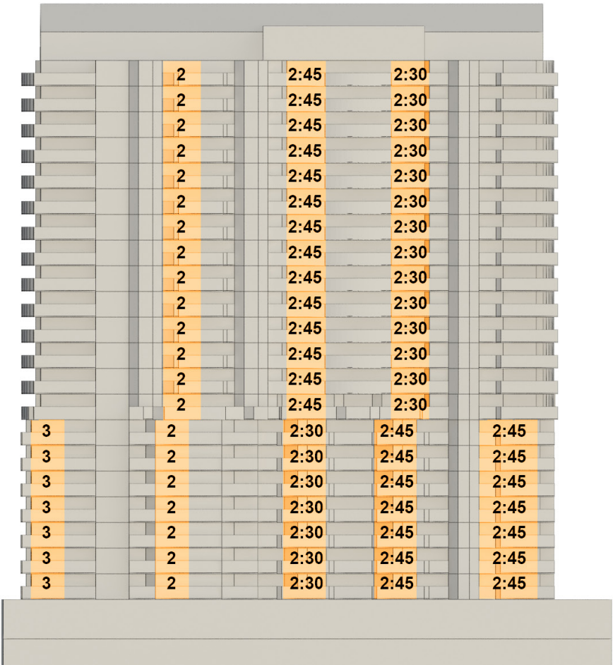
Hours of Solar access to Living Rooms
